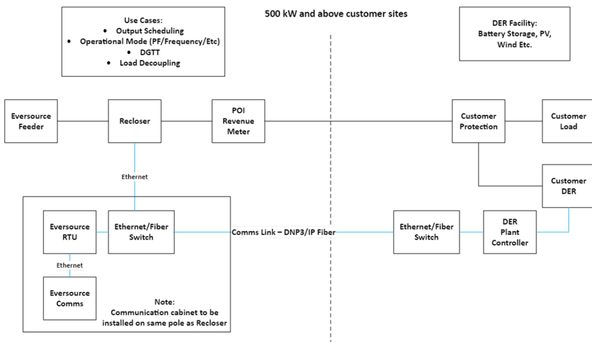
Example Single Line Diagram of OH Design
