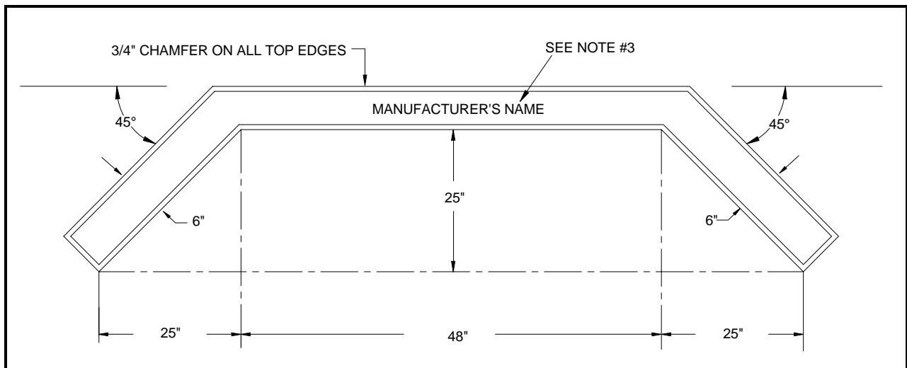
Figure 1 - Retaining Wall Top View (Top View)
